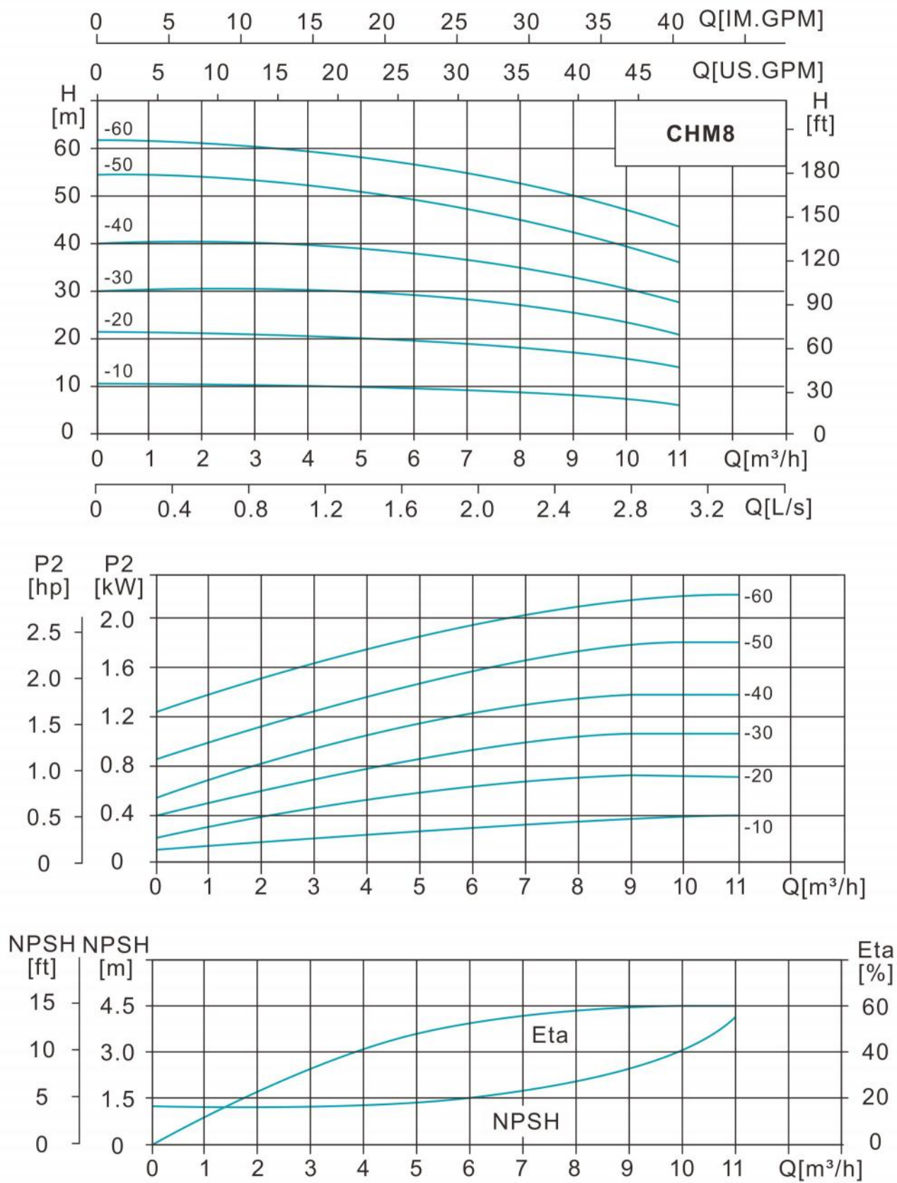
Performance Curve Of CHM
