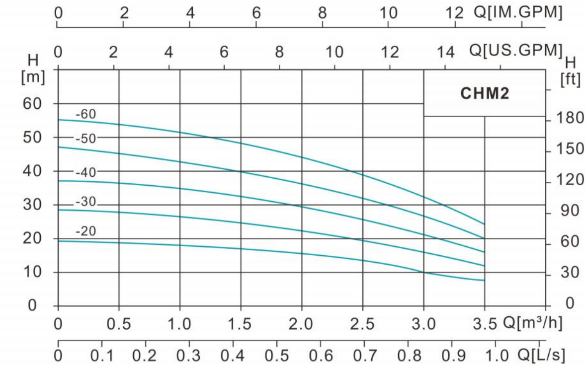
Performance Curve Of CHM
