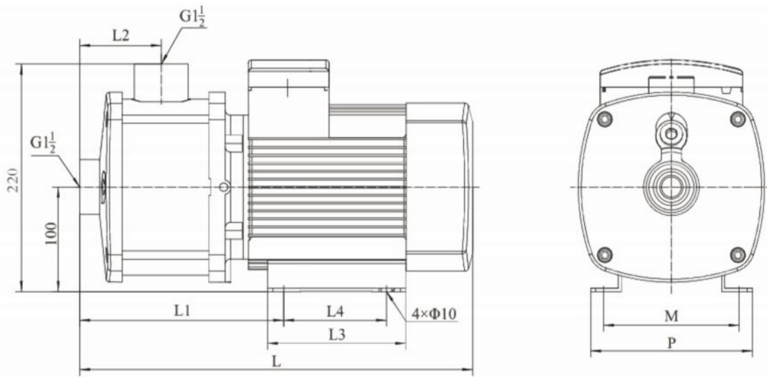
Installation Drawing Of CHM
