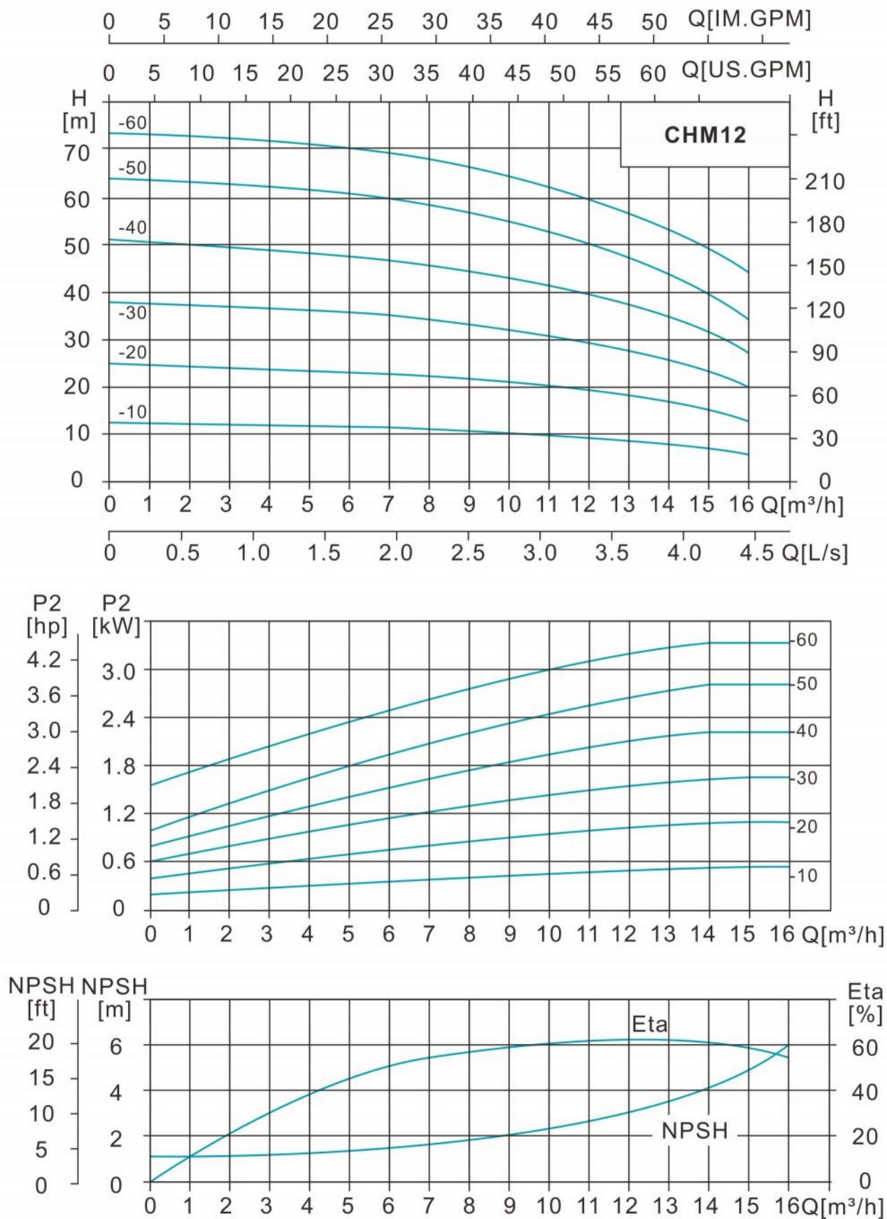
Performance Curve Of CHM
