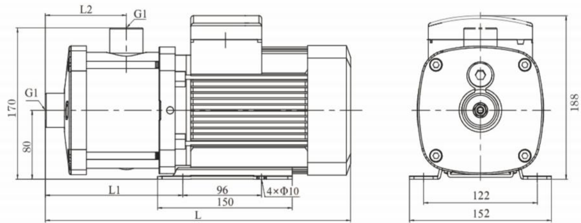
Installation Drawing Of CHM
